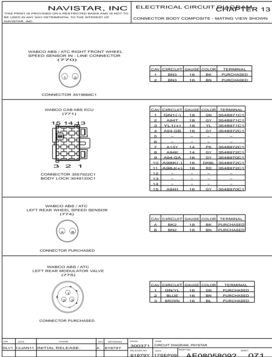
Figure 277 Connector Composites (770 / 771 / 774 / 775)
