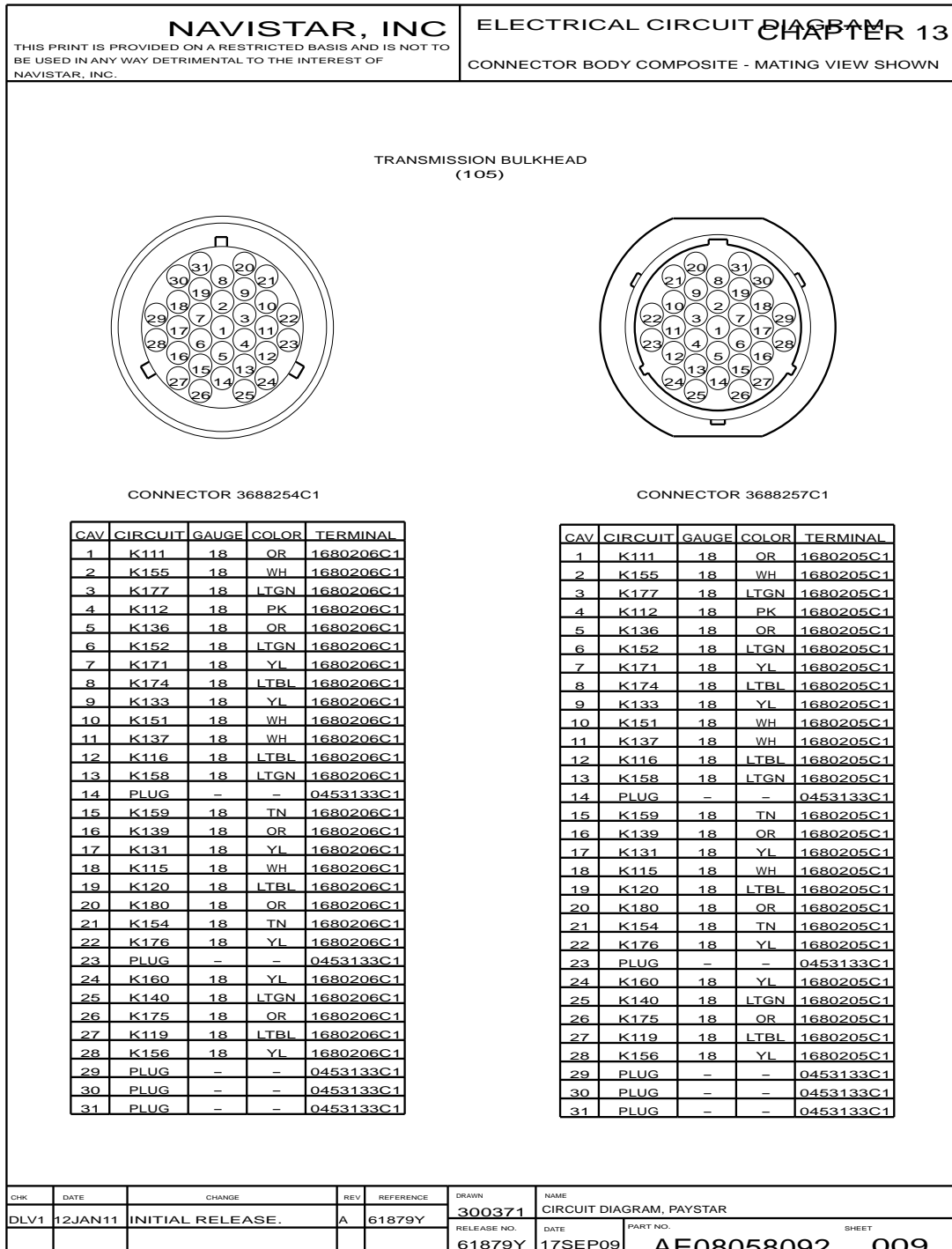
Figure 199 Connector Composites (105)
