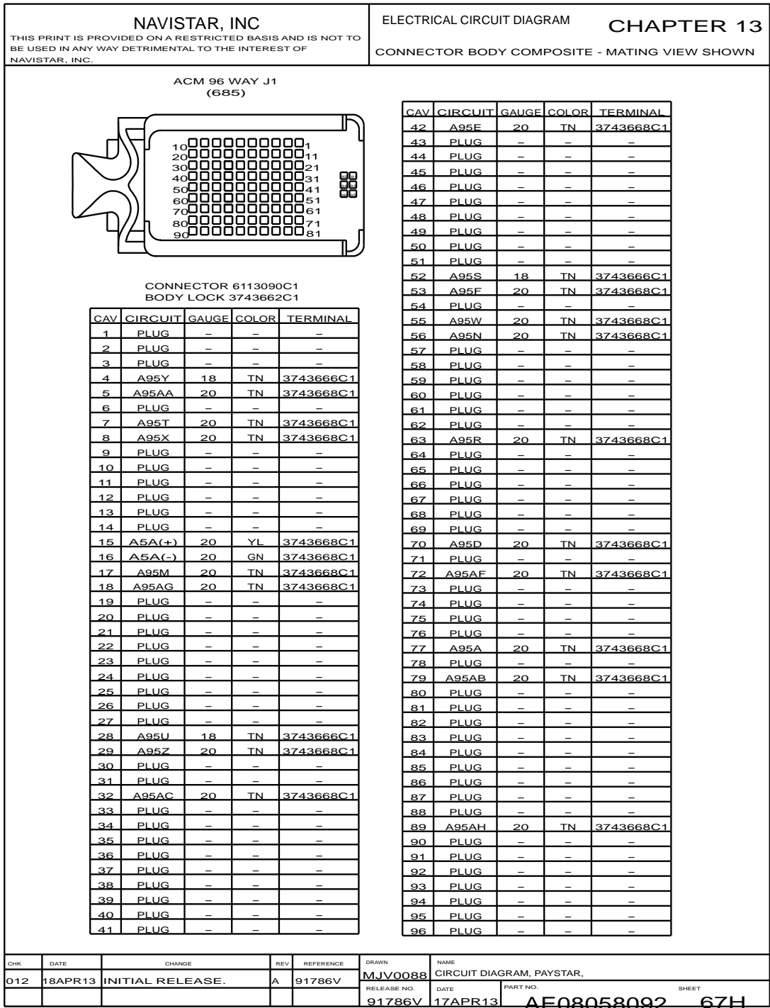
Figure 272 Connector Composites (685)
