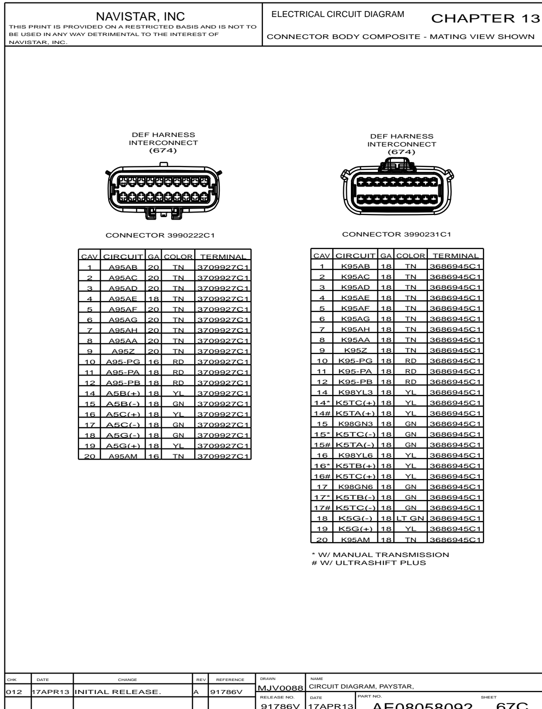
Figure 267 Connector Composites (674)
