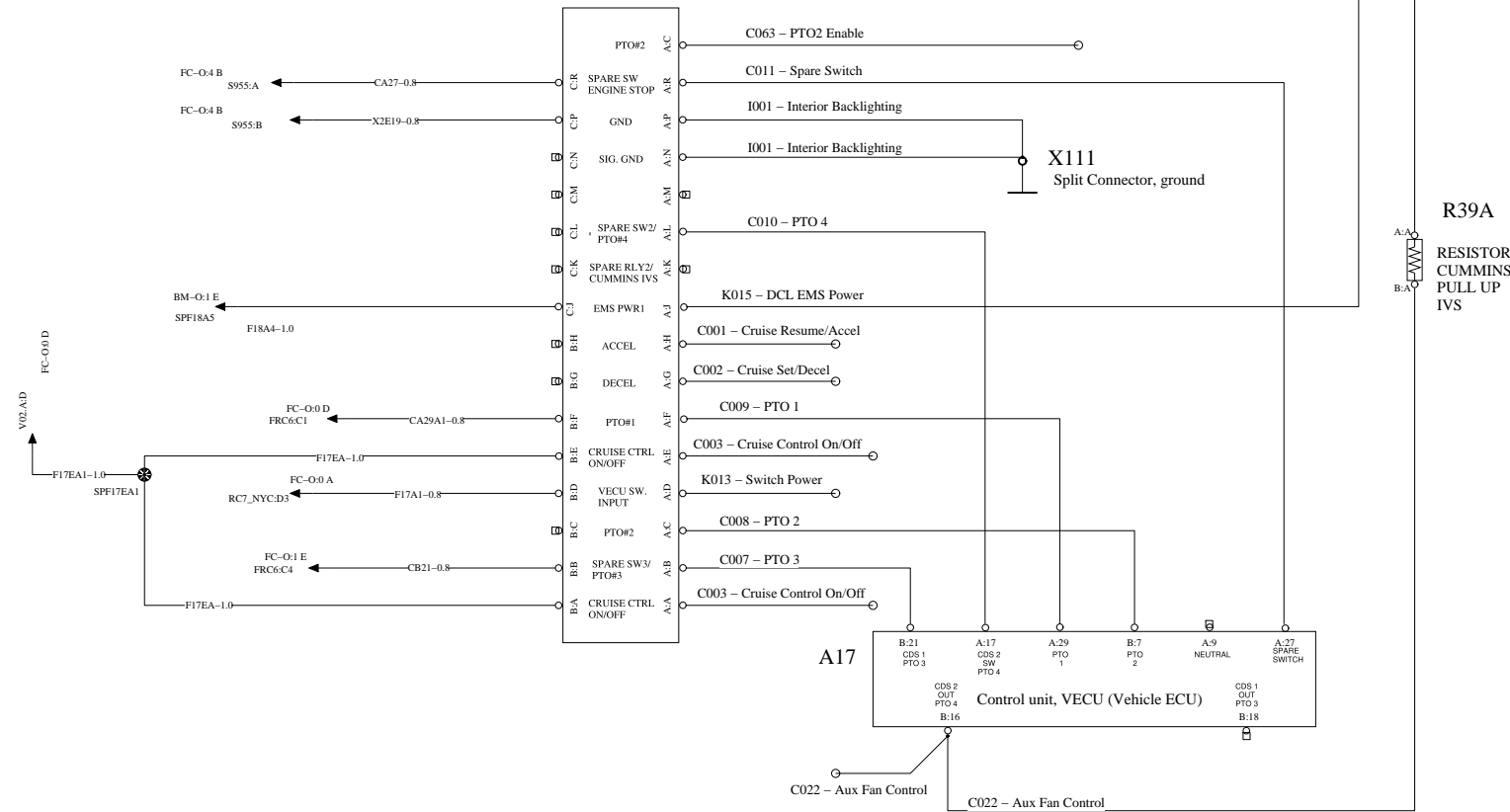
X21A Socket, Body builder connector
